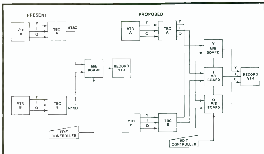
Figure 1. WNEV-TV edit suite flow chart.
