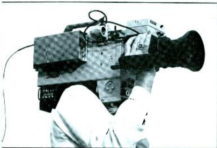
Camera person shooting with portable, battery-operated ENG/EFP fiber-optic video and audio transmitter affixed to camera.
