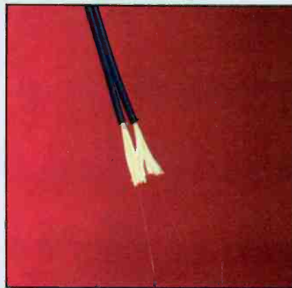
Dual-fiber tight-buffered cable stripped before connectorization with exposed fiber and yellow Kevlar.
